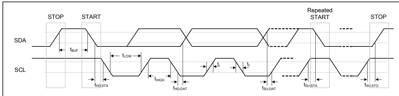
Figure 5-11 I2C Bus Timing
