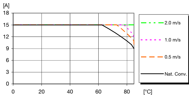
Available load current vs. ambient air temperature and airflow at V_i = 5.0\text{ V} , V_{OUT} = 3.3\text{ V} . See Thermal Consideration section.
