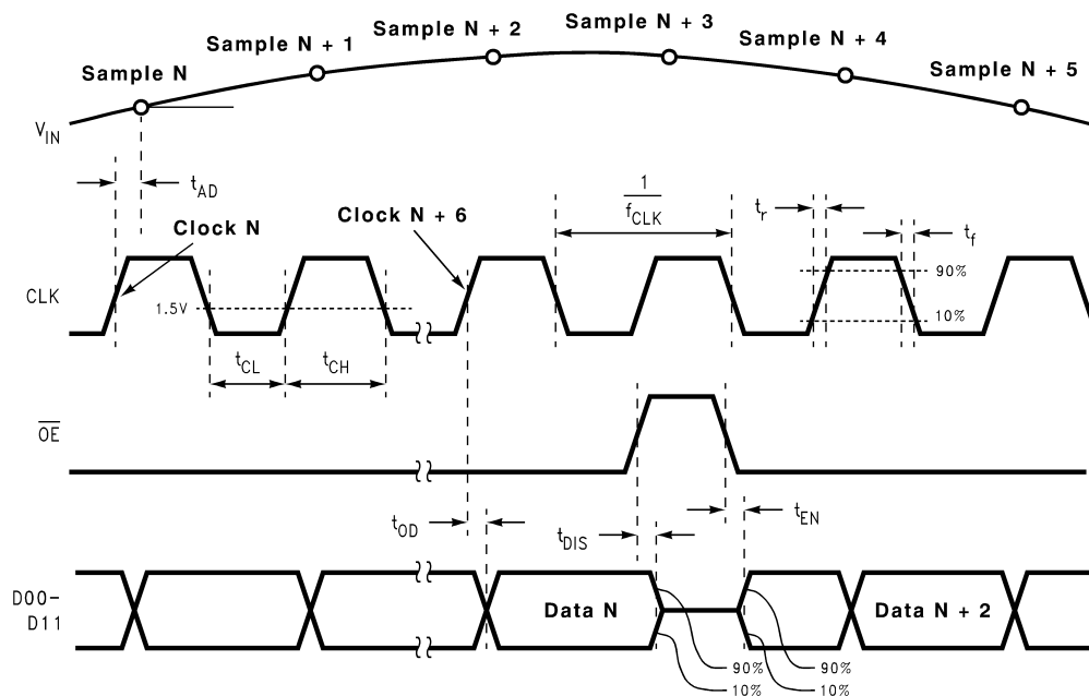
Output Timing
