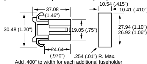
Recommended Panel Mounting Hole (.04" / .078" thick panel)
