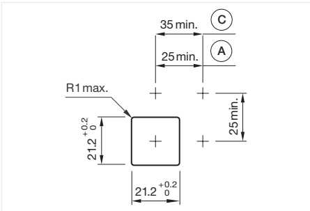
Mounting cut-outs [mm] A = Solder/Plug-in terminal 2.8 mm x 0.5 mm C = Screw terminal
