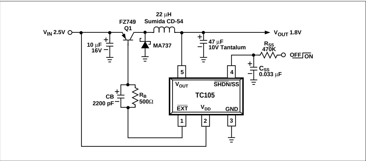
Figure 3. Regulator Using PNP Transistor
