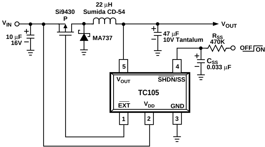
Figure 4. Regulator Using P-Channel MOSFET
