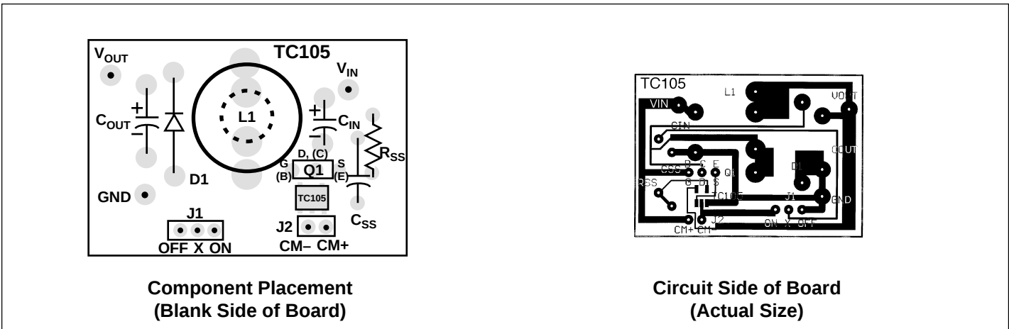
Figure 6. Component Placement
