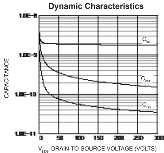
Figure 2, Typical Capacitance vs. Drain-to-Source Voltage
