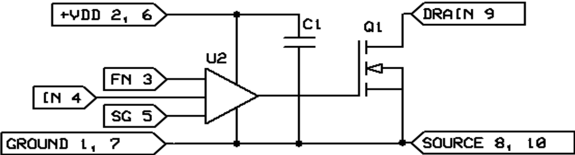
Figure 3, DRF1202 Test Circuit
