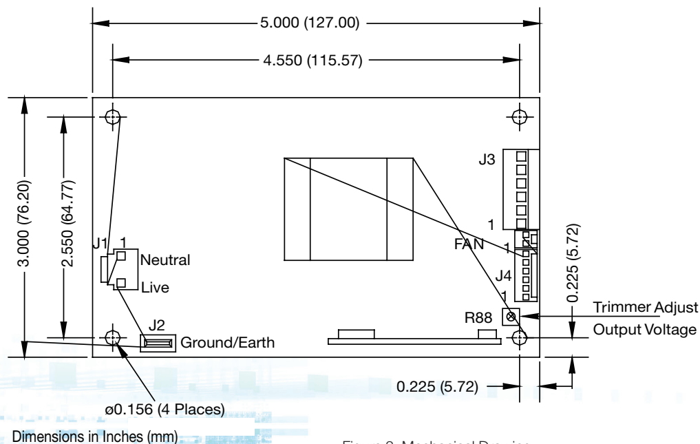
Figure 2: Mechanical Drawing
