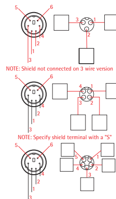
CUSTOM WIRING FOR CONNECTOR CONFIGURATION 3, 4 AND 6
