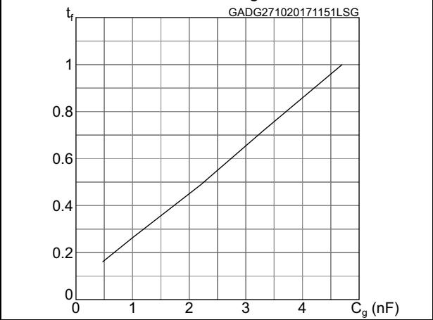
Figure 15. Gate driver low side fall time normalized vs C g = 4.7nF
