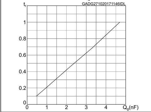
Figure 14. Gate driver low side rise time normalized vs C g = 4.7nF
