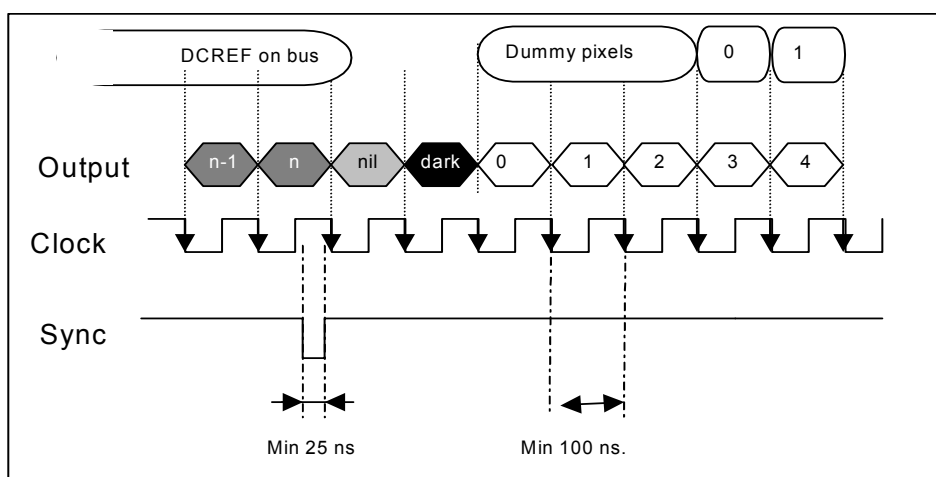
Figure 20 : timing of X shift register and pixels read-out
