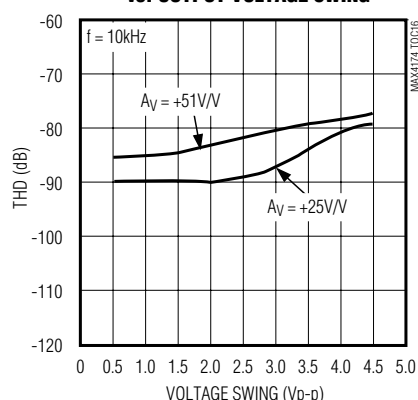
TOTAL HARMONIC DISTORTION vs. OUTPUT VOLTAGE SWING
