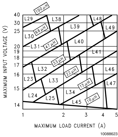
FIGURE 5. LM2678-12
