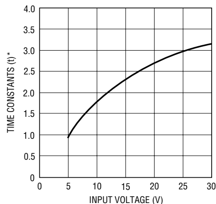
Delay Time
