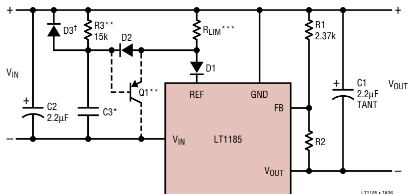
Time Delayed Start-Up
