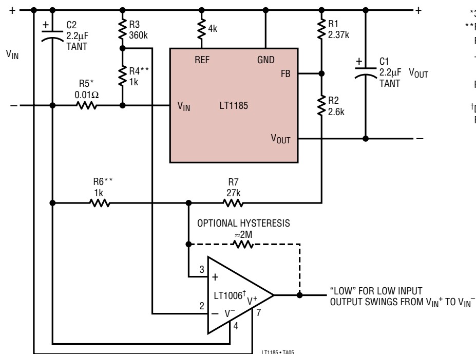
Low Input Voltage Monitor Tracks Dropout Characteristics
