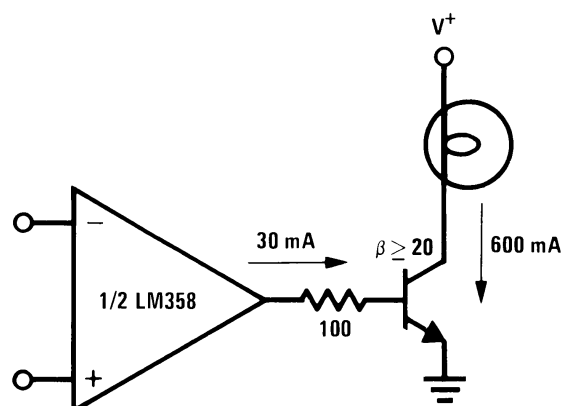
Figure 8-6. Lamp Driver
