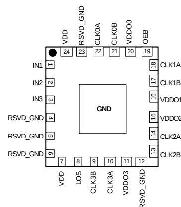
Si5330 Transparent Top View
