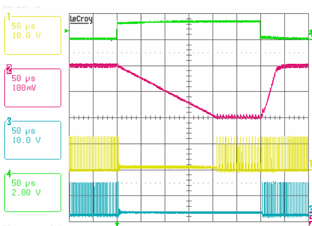
FIGURE 46. 2-PHASE CPU MODE DEEPER SLEEP MODE ENTRY/EXIT, I_O = 1.5A , HFM VID = 1.075V , LFM VID = 0.875V , DEEPER SLEEP VID = 0.875V , Ch1: PHASE1, Ch2: V_0 , Ch3: PHASE2, CH4: DPRSLPVR
