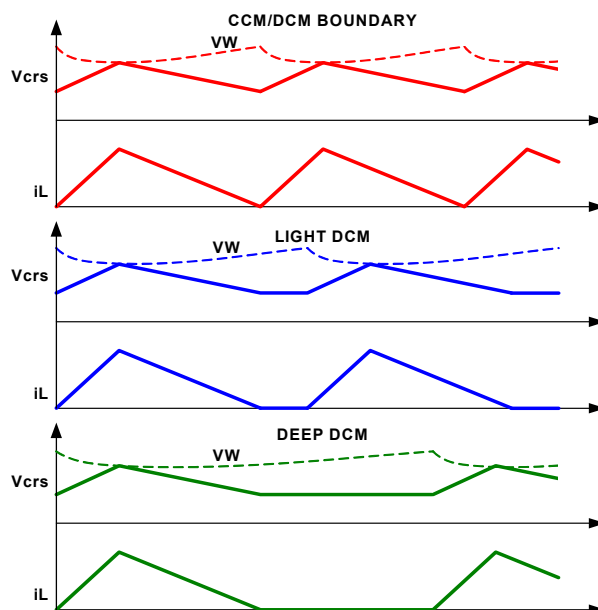
FIGURE 9. PERIOD STRETCHING
