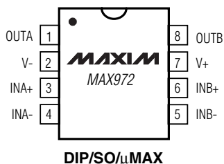
DIP/SO/μMAX
