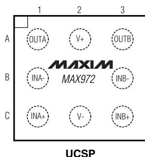
UCSP
