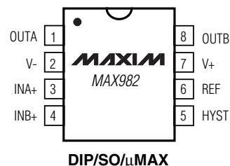
DIP/SO/μMAX
