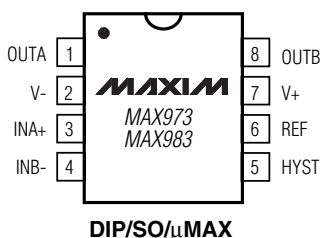
DIP/SO/μMAX
