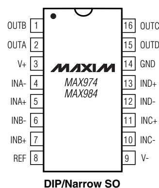
DIP/Narrow SO
