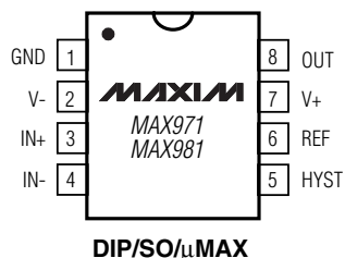
DIP/SO/μMAX
