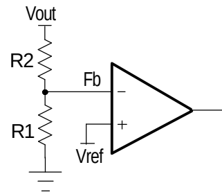
Voltage divider
