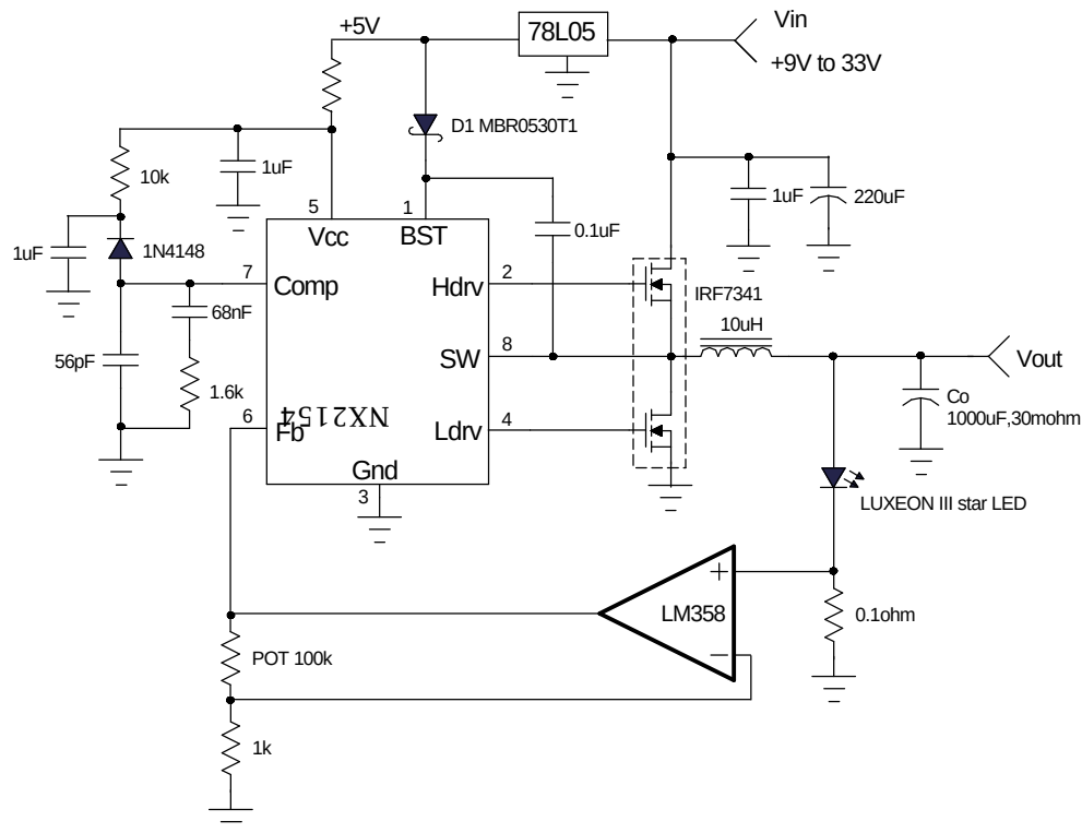
Figure 10 - NX2154 LED application
