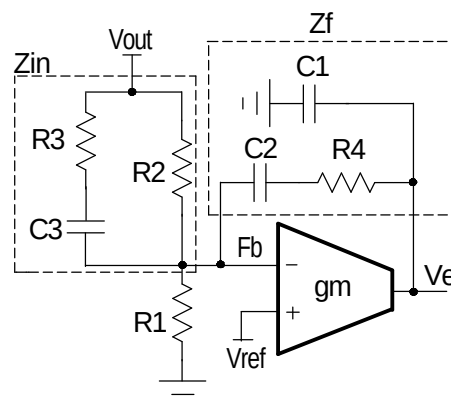
Figure 3 - Type III compensator using transconductance amplifier
