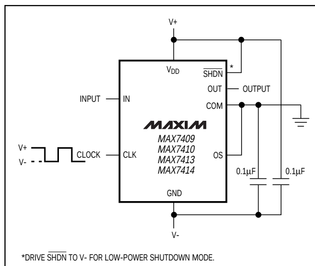
Figure 4. Dual-Supply Operation
