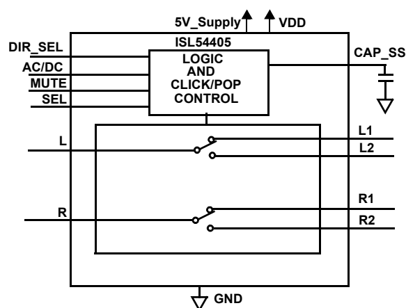
FIGURE 1. ISL54405 BLOCK DIAGRAM
