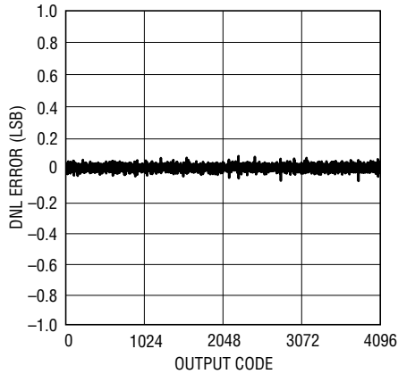
LTC2259-12: Differential Nonlinearity (DNL)
