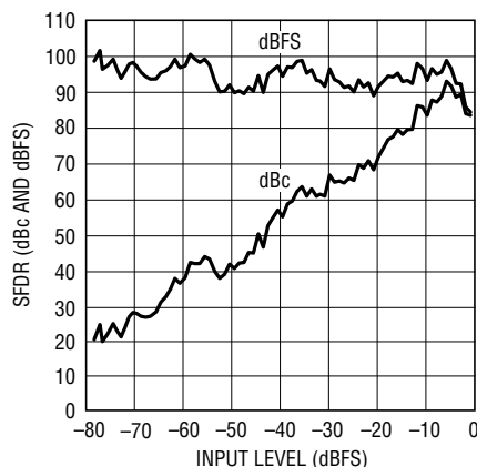
LTC2261-12: SFDR vs Input Level, f_{IN} = 70\text{MHz} , 2V Range, 125Mps
