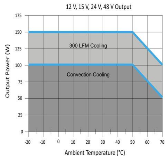
Figure 1 - Output Power Vs. Temperature
