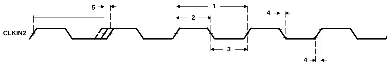
Figure 7-32. CLKIN2 Timing
