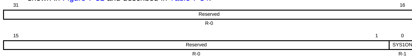
Figure 7-31. SYSCLK Status Register [Hex Address: 029C 0150]
