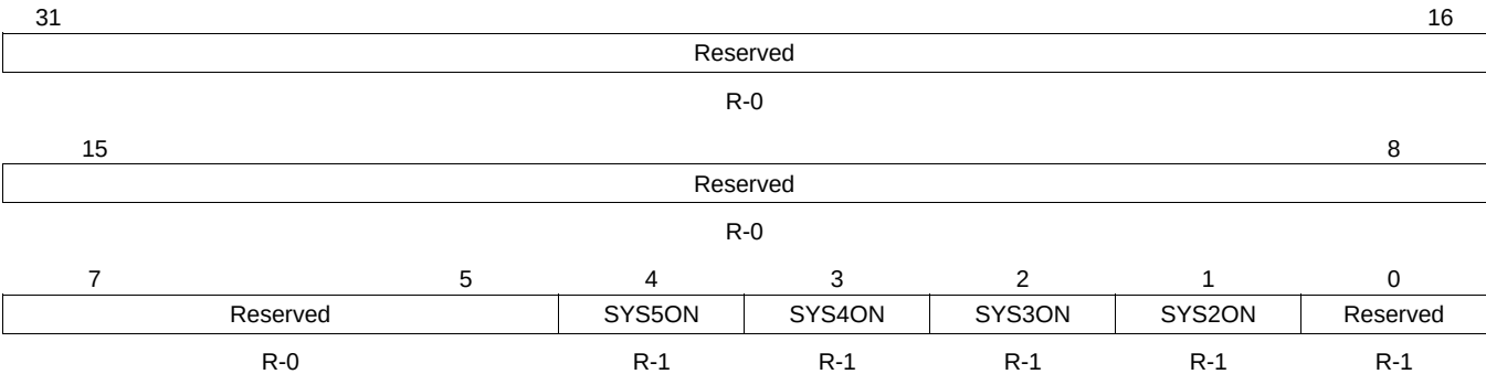
Figure 7-22. SYSClk Status Register (SYSTAT) [Hex Address: 029A 0150]
