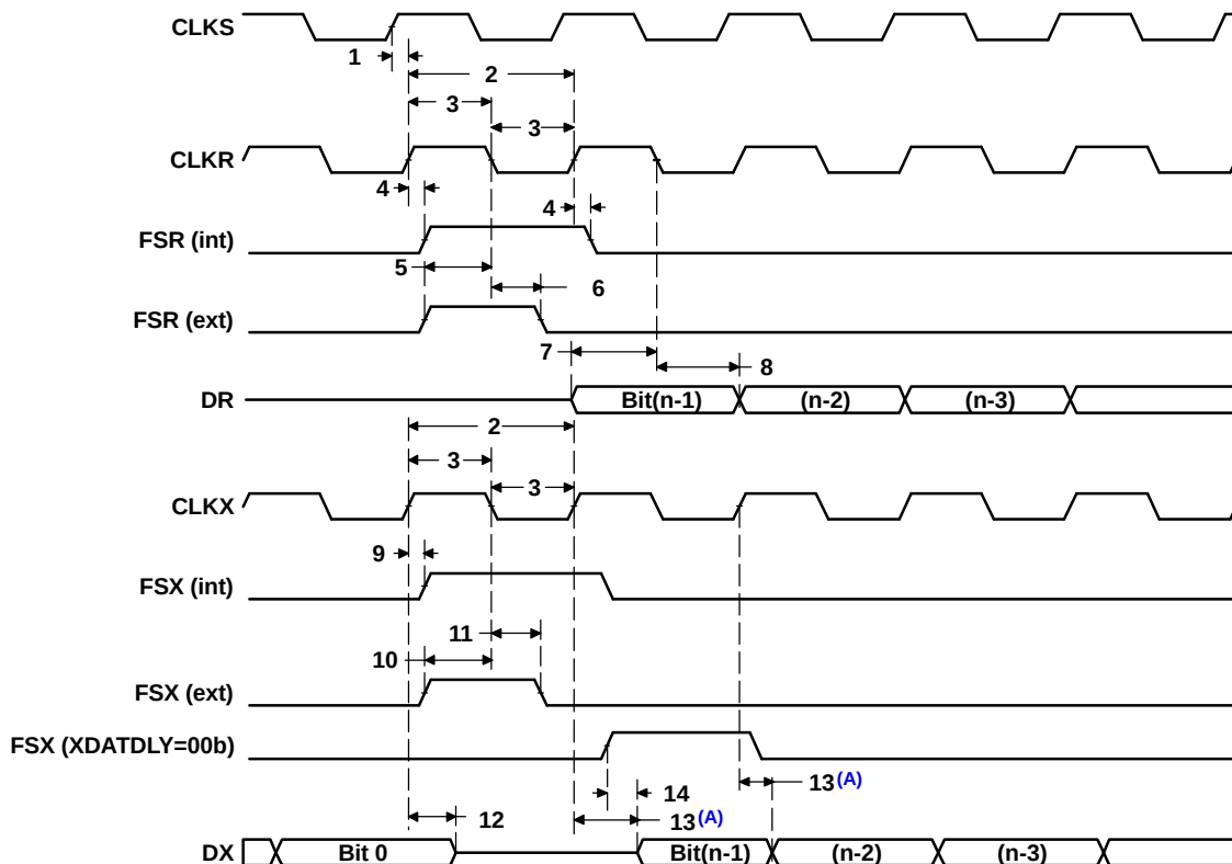
Figure 7-54. McBSP Timing (B)
