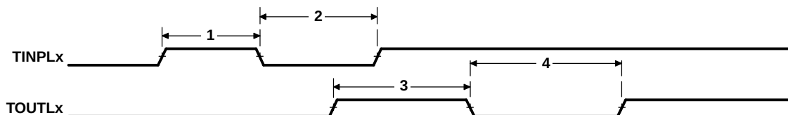
Figure 7-75. Timer Timing
