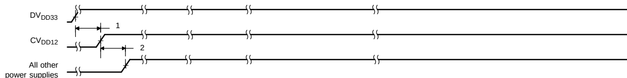
Figure 7-6. Power-Supply Sequence (Option 2)
