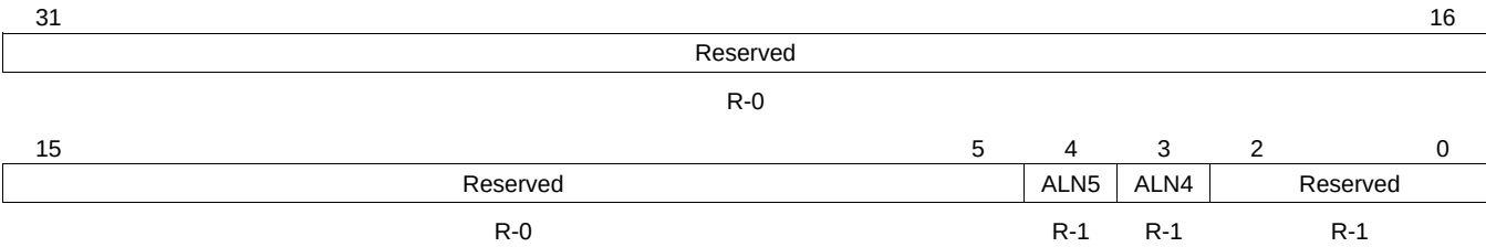
Figure 7-20. PLL Controller Clock Align Control Register (ALNCTL) [Hex Address: 029A 0140]
