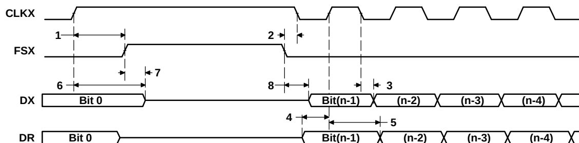
Figure 7-58. McBSP Timing as SPI Master or Slave: CLKSTP = 10b, CLKXP = 1
