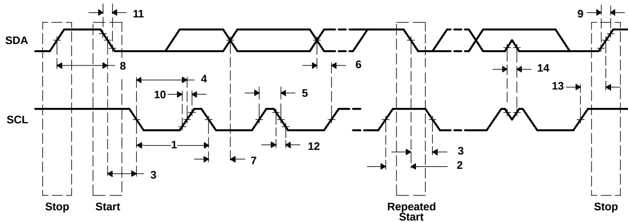
Figure 7-44. I2C Receive Timings
