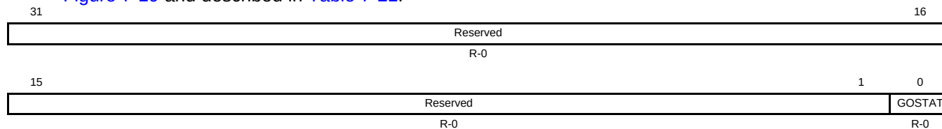
Figure 7-19. PLL Controller Status Register (PLLSTAT) [Hex Address: 029A 013C]
