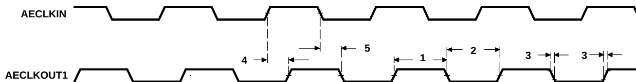
Figure 7-34. AECLKOUT Timing for the EMIFA Module
