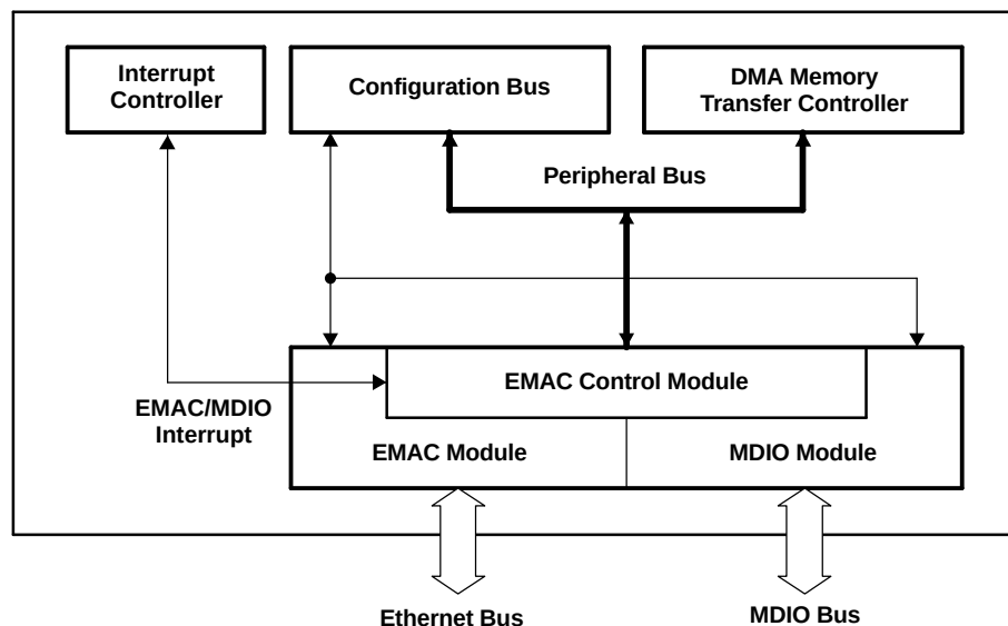
Figure 7-60. EMAC, MDIO, and EMAC Control Modules
