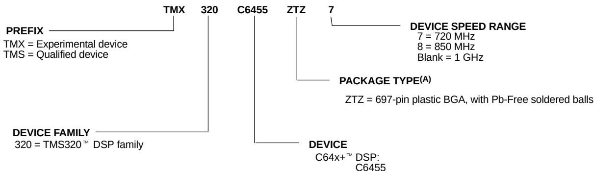
Figure 2-13. TMS320C64x+™ DSP Device Nomenclature (including the TMS320C6455 DSP)
