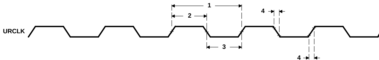
Figure 7-81. URCLK Timing
