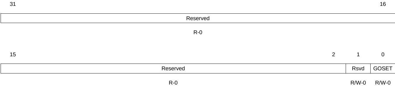
Figure 7-18. PLL Controller Command Register (PLLCMD) [Hex Address: 029A 0138]
