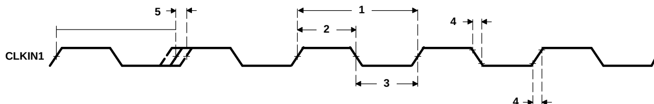
Figure 7-23. CLKIN1 Timing
