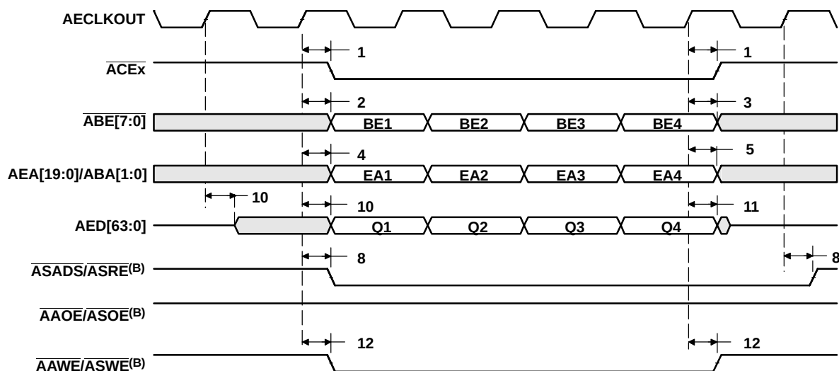
Figure 7-38. Programmable Synchronous Interface Read Timing for EMIFA (With Read Latency = 2) (A)
