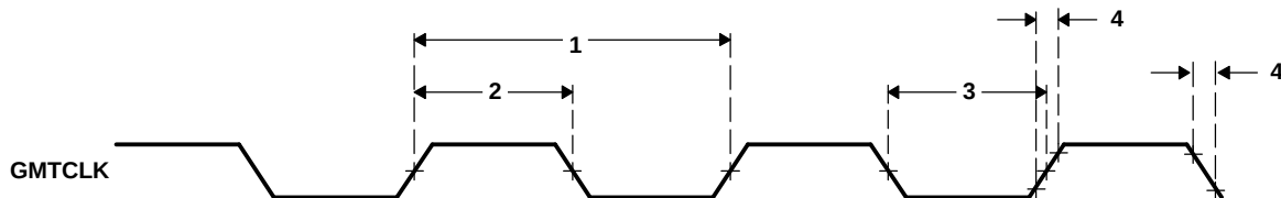
Figure 7-63. GMTCLK Timing (EMAC – Transmit) [GMII Operation]
