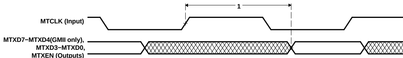
Figure 7-65. EMAC Transmit Interface Timing [MII and GMII Operation]
