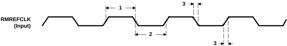
Figure 7-67. RMREFCLK Timing
