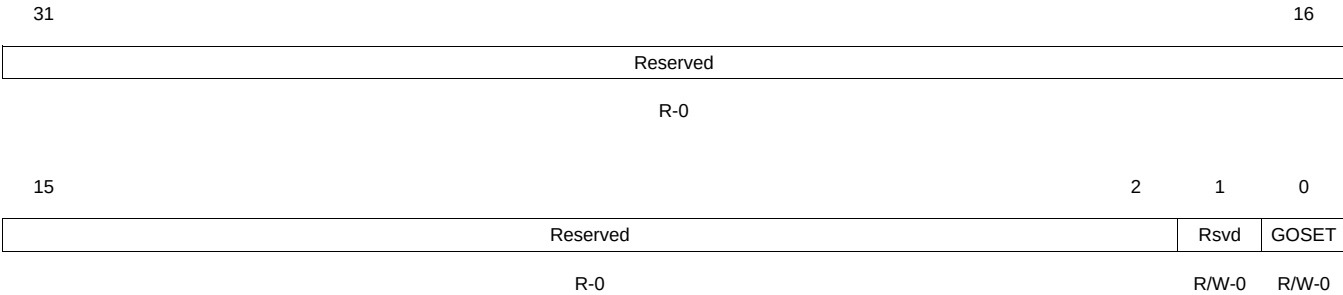
Figure 7-27. PLL Controller Command Register (PLLCMD) [Hex Address: 029C 0138]
