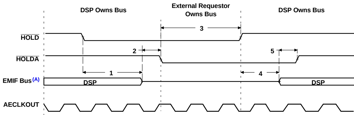
Figure 7-41. \overline{\text{HOLD}}/\overline{\text{HOLDA}} Timing for EMIFA
