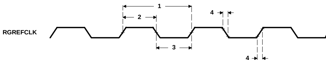
Figure 7-68. RGMIIREFCLK Timing
