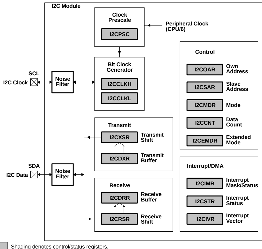
Figure 7-43. I2C Module Block Diagram
