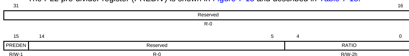
Figure 7-15. PLL Pre-Divider Register (PREDIV) [Hex Address: 029A 0114]
