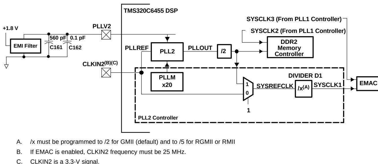
Figure 7-25. PLL2 Block Diagram
