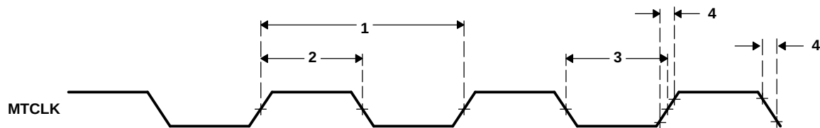
Figure 7-62. MTCLK Timing (EMAC – Transmit) [MII and GMII Operation]
