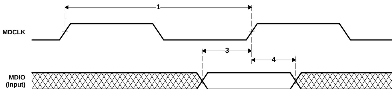
Figure 7-73. MDIO Input Timing
