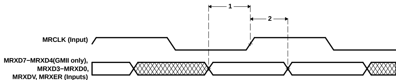
Figure 7-64. EMAC Receive Interface Timing [MII and GMII Operation]
