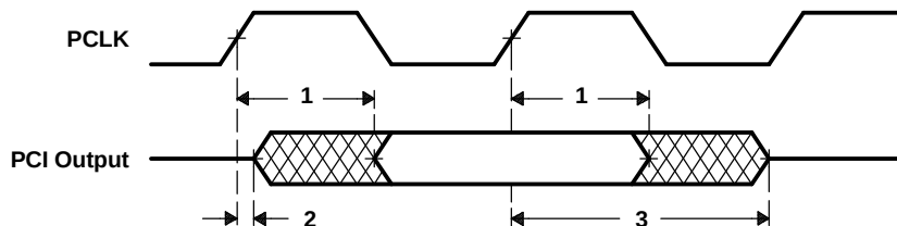
Figure 7-79. PCI Output Timing (33-/66-MHz)
