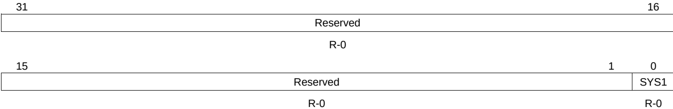
Figure 7-30. PLLDIV Divider Ratio Change Status Register (DCHANGE) [Hex Address: 029C 0144]
