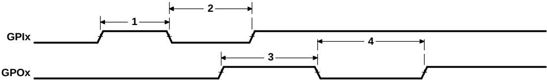
Figure 7-84. GPIO Port Timing
