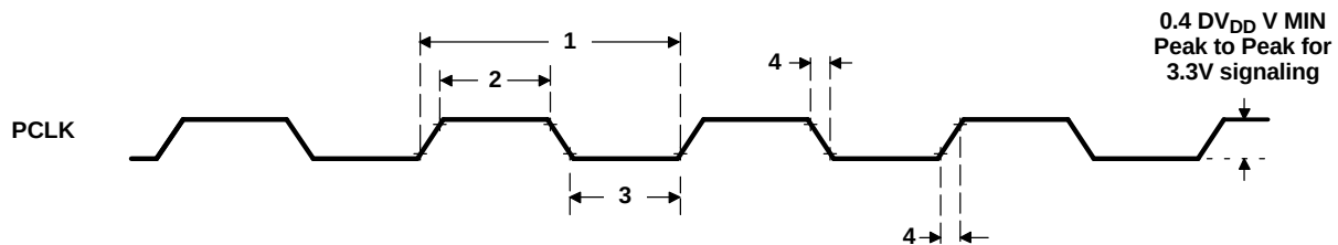
Figure 7-76. PCLK Timing
