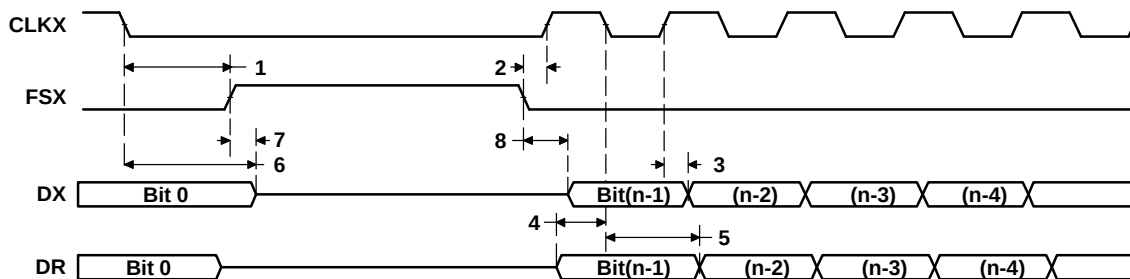
Figure 7-56. McBSP Timing as SPI Master or Slave: CLKSTP = 10b, CLKXP = 0
