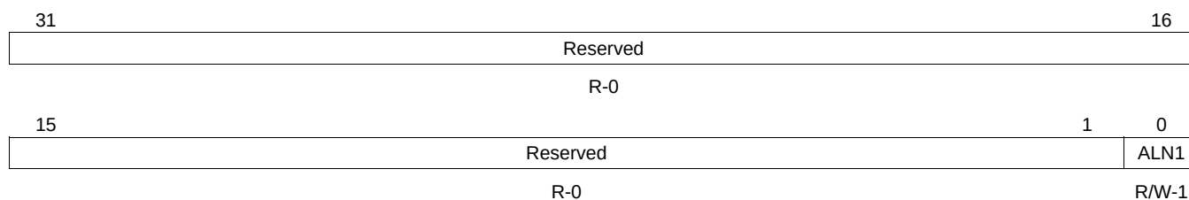
Figure 7-29. PLL Controller Clock Align Control Register (ALNCTL) [Hex Address: 029C 0140]
