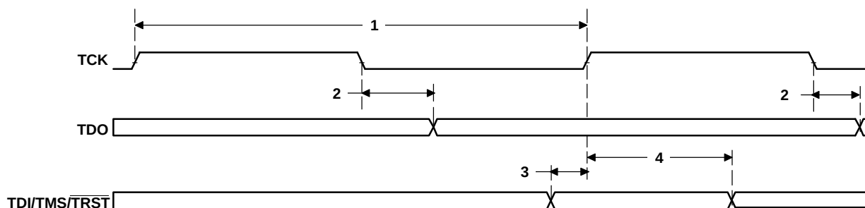
Figure 7-85. JTAG Test-Port Timing
