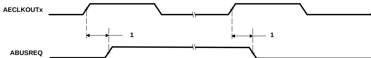
Figure 7-42. BUSREQ Timing for EMIFA
