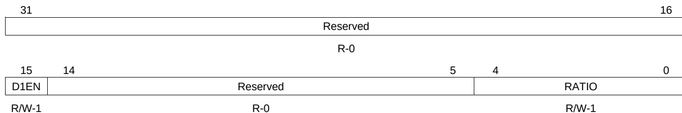
Figure 7-26. PLL Controller Divider 1 Register (PLLDIV1) [Hex Address: 029C 0118]
