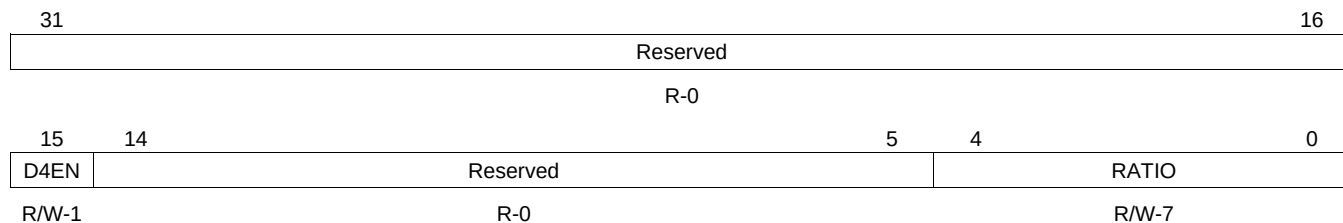
Figure 7-16. PLL Controller Divider Register 4 (PLLDIV4) [Hex Address: 029A 0160]
