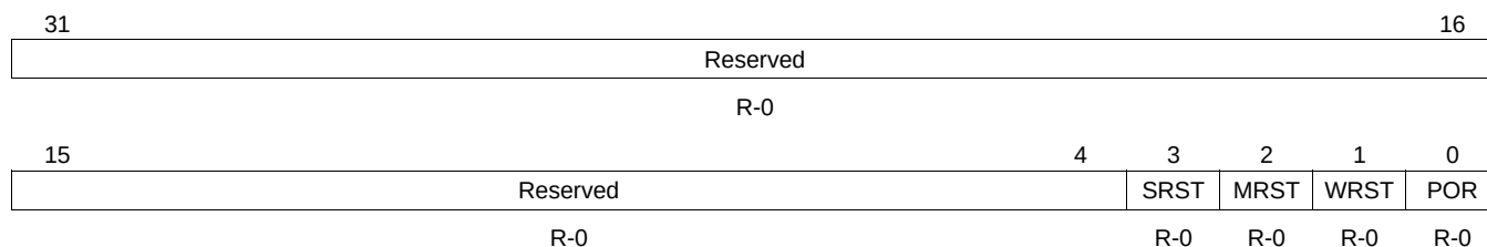
Figure 7-8. Reset Type Status Register (RSTYPE) [Hex Address: 029A 00E4]
