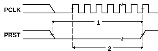
Figure 7-77. PCI Reset ( \overline{\text{PRST}} ) Timing
