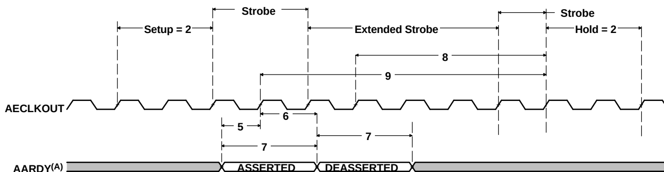
Figure 7-36. Asynchronous Memory Write Timing for EMIFA
