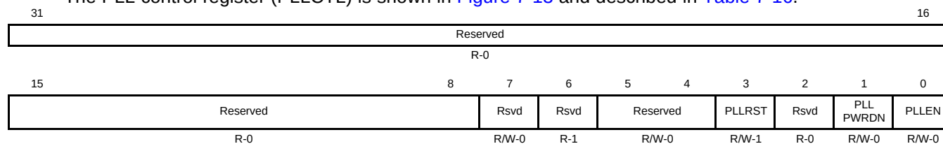
Figure 7-13. PLL1 Control Register (PLLCTL) [Hex Address: 029A 0100]
