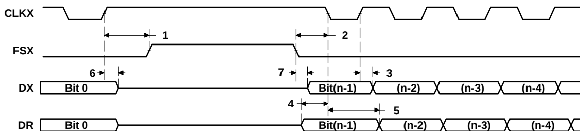
Figure 7-59. McBSP Timing as SPI Master or Slave: CLKSTP = 11b, CLKXP = 1
