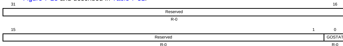
Figure 7-28. PLL Controller Status Register (PLLSTAT) [Hex Address: 029C 013C]
