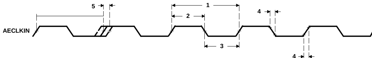
Figure 7-33. AECLKIN Timing for EMIFA
