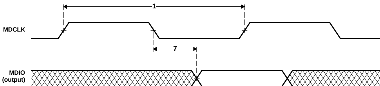
Figure 7-74. MDIO Output Timing
