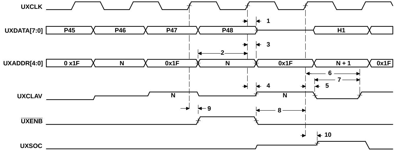
Figure 7-82. UTOPIA Slave Transmit Timing (A)
