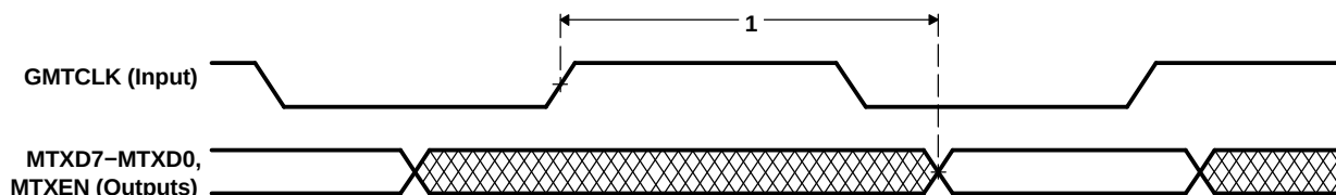
Figure 7-66. EMAC Transmit Interface Timing [GMII Operation]
