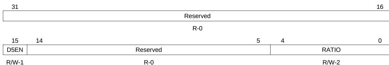
Figure 7-17. PLL Controller Divider Register 5 (PLLDIV5) [Hex Address: 029A 0164]
