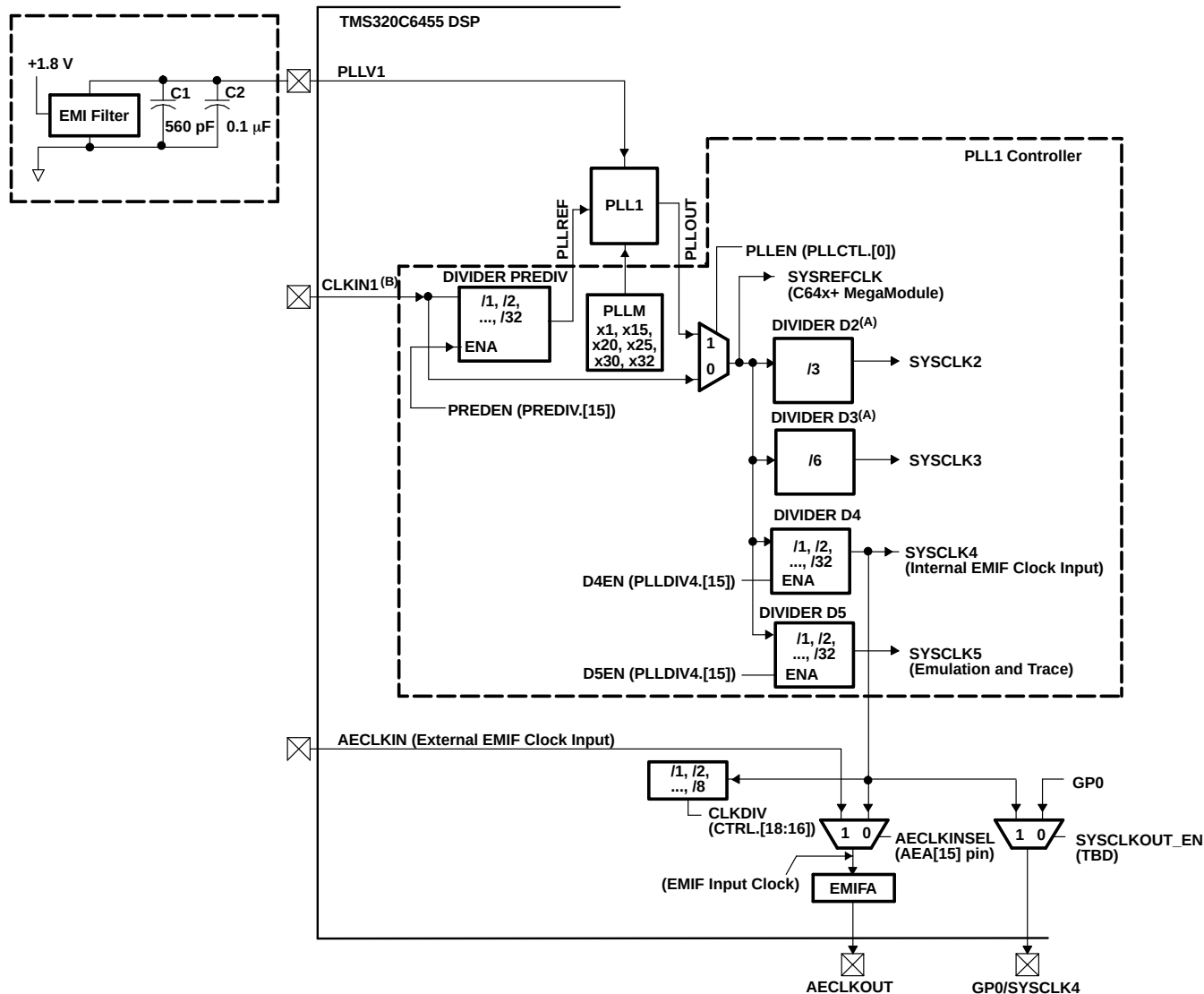
Figure 7-12. PLL1 and PLL1 Controller
