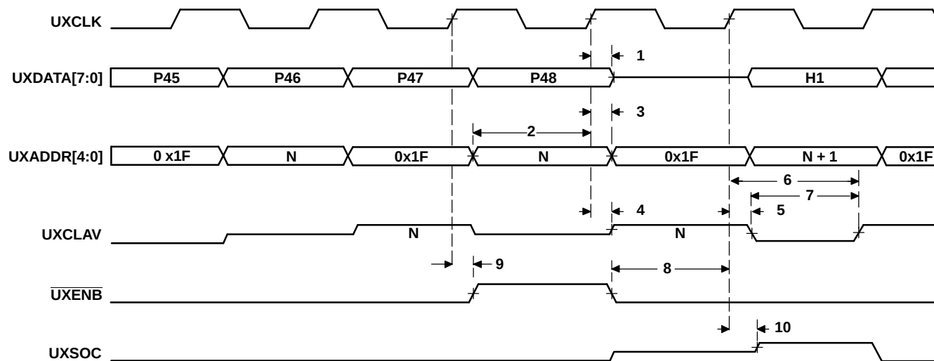
Figure 7-83. UTOPIA Slave Receive Timing (A)
