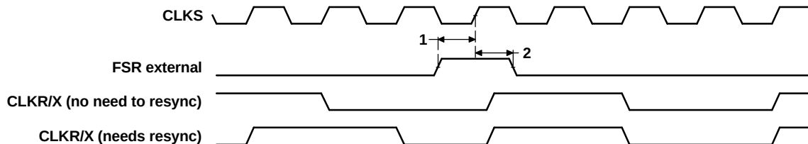
Figure 7-55. FSR Timing When GSYNC = 1
