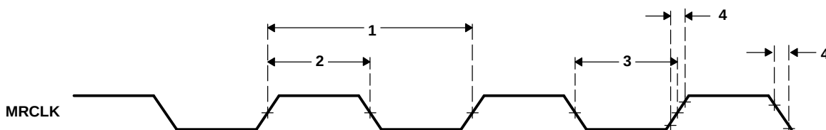
Figure 7-61. MRCLK Timing (EMAC – Receive) [MII and GMII Operation]
