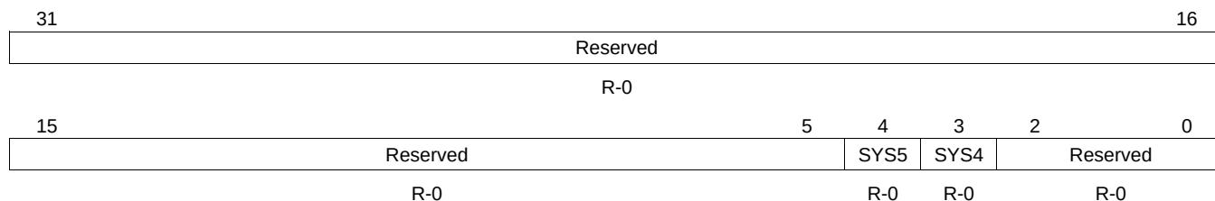
Figure 7-21. PLLDIV Divider Ratio Change Status Register (DCHANGE) [Hex Address: 029A 0144]
