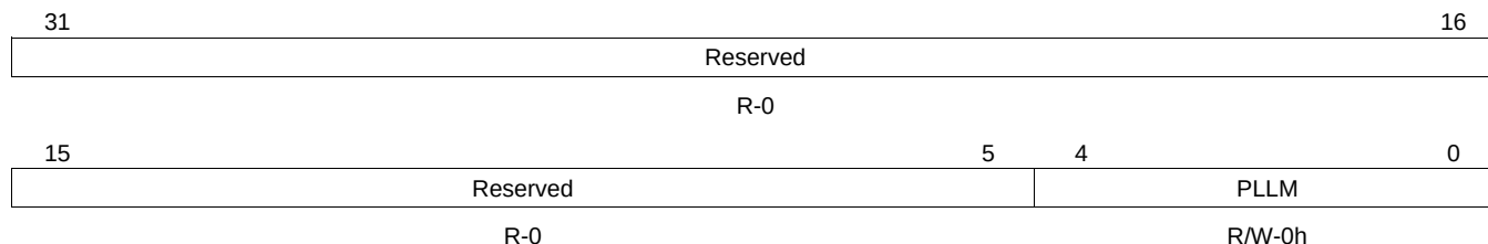
Figure 7-14. PLL Multiplier Control Register (PLLM) [Hex Address: 029A 0110]
