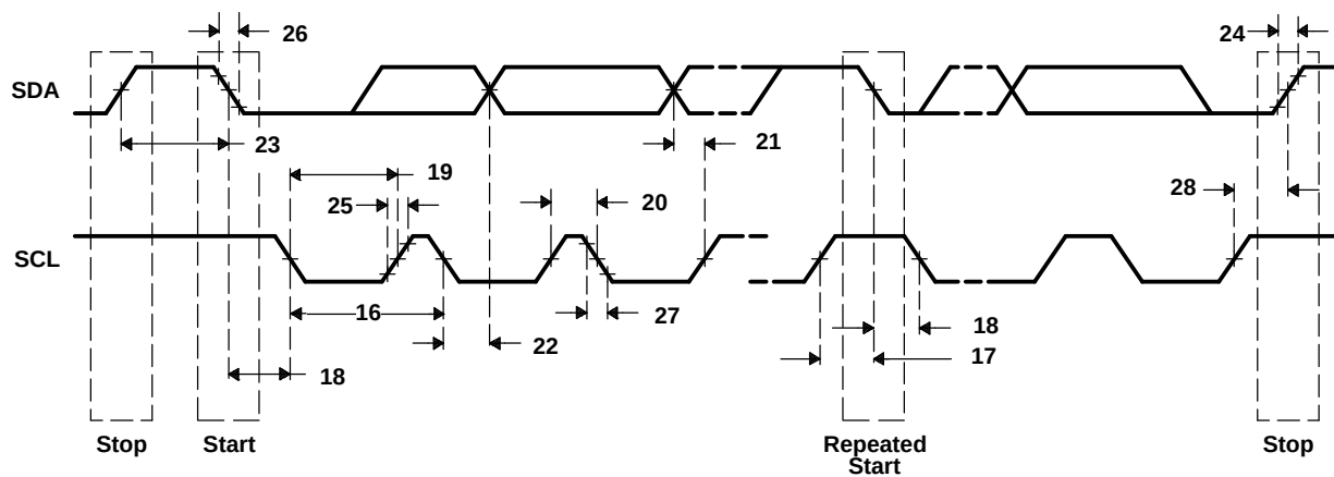
Figure 7-45. I2C Transmit Timings
