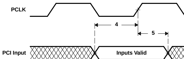
Figure 7-78. PCI Input Timing (33-/66-MHz)
