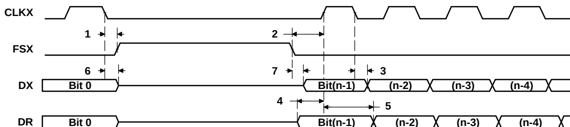
Figure 7-57. McBSP Timing as SPI Master or Slave: CLKSTP = 11b, CLKXP = 0
