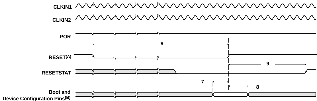
Figure 7-10. Warm Reset and Max Reset Timing
