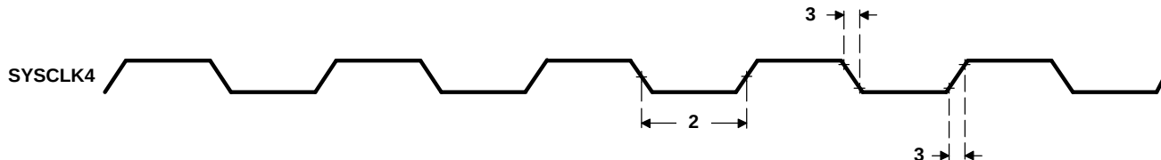
Figure 7-24. SYSCLK4 Timing
