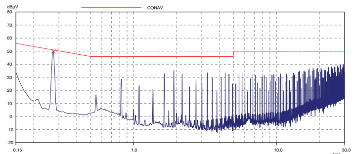
Graph 1. Conducted emissions performance with filter, Negative Line, CISPR 22, Class B, full load, for UEI30-Q33-Q48N-C
