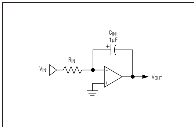
Figure 10. Long-Time Constant Integrator—With R_{IN} = 10^{11}\Omega , the time constant of this integrator is 100,000s. Since the input voltage is converted to a current by R_{IN} , the input voltage can far exceed the power-supply range.
