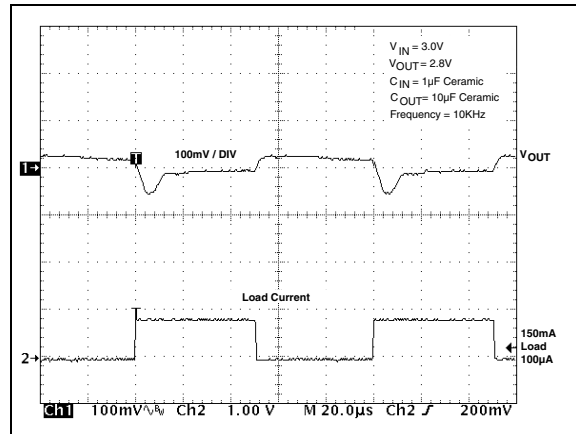
FIGURE 5-17: SHUTDOWN DELAY
