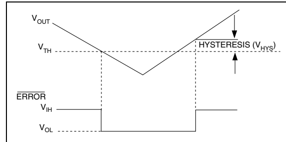
FIGURE 3-2: ERROR OUTPUT OPERATION
