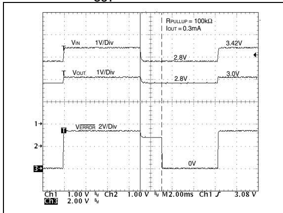
FIGURE 5-19: V_{OUT} TO ERROR DELAY
