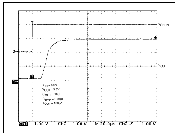
FIGURE 5-18: SHUTDOWN WAKE-UP TIME
