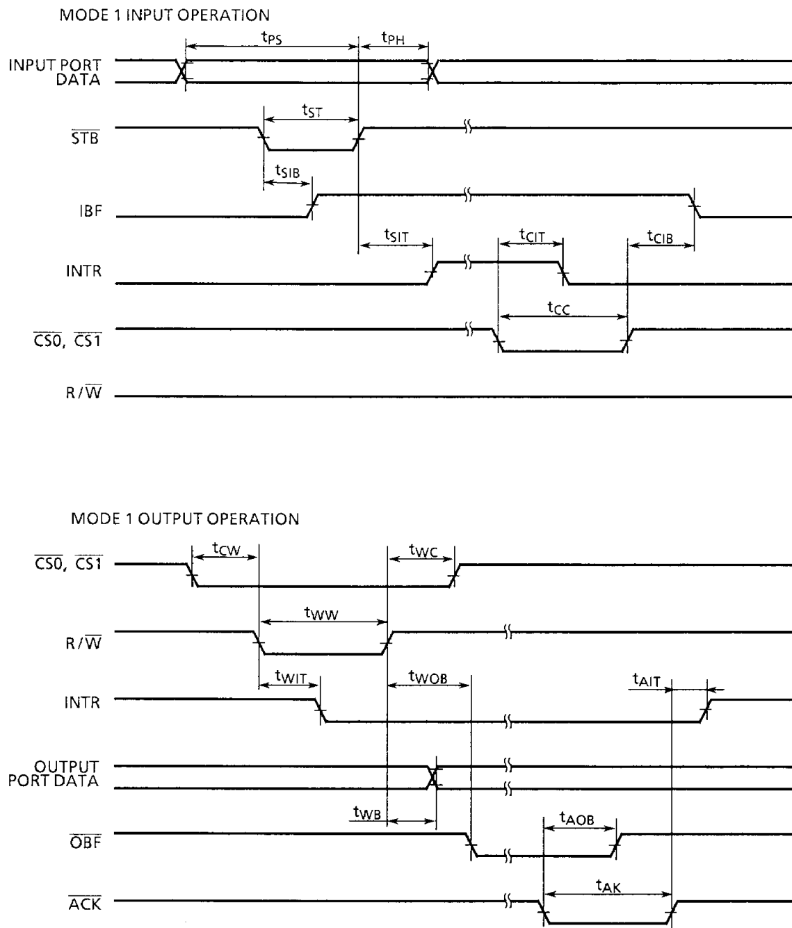
Figure 8.1 TMP82C255A Timing diagram (2)
