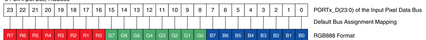
Figure 13. Pixel Mapping
