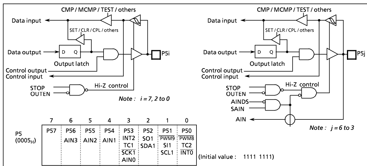
Figure 2-6. Ports P5
