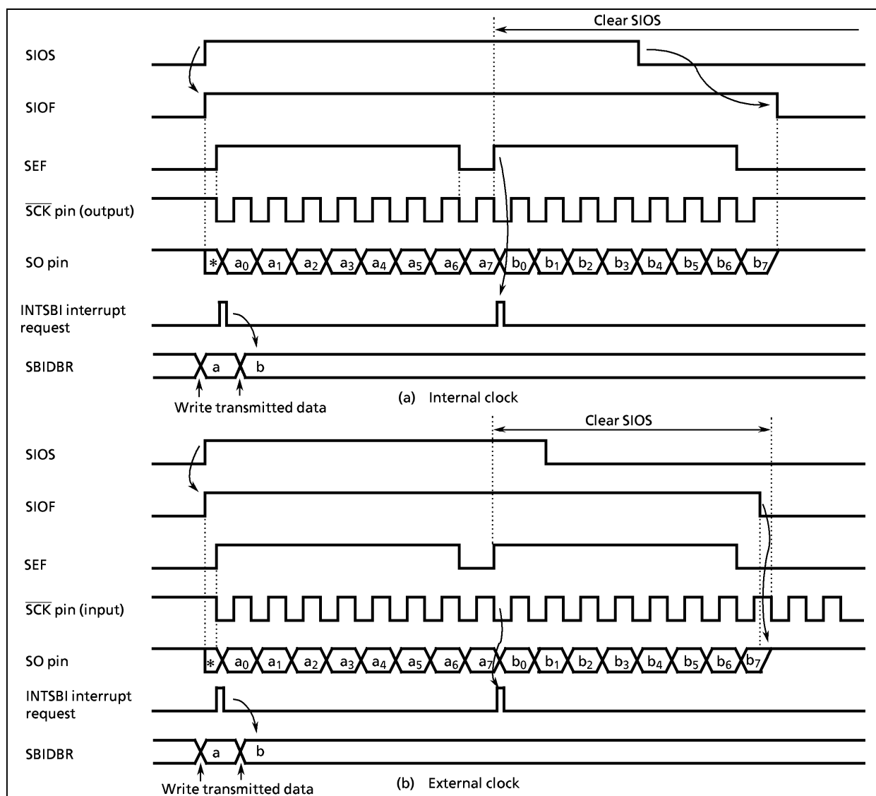
Figure 2-47. Transfer mode
