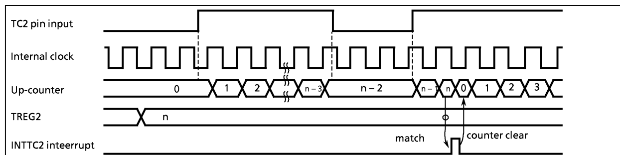
Figure 2-21. Window mode timing chart
