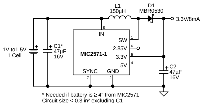
Single-Cell to 3.3V DC-to-DC Converter
