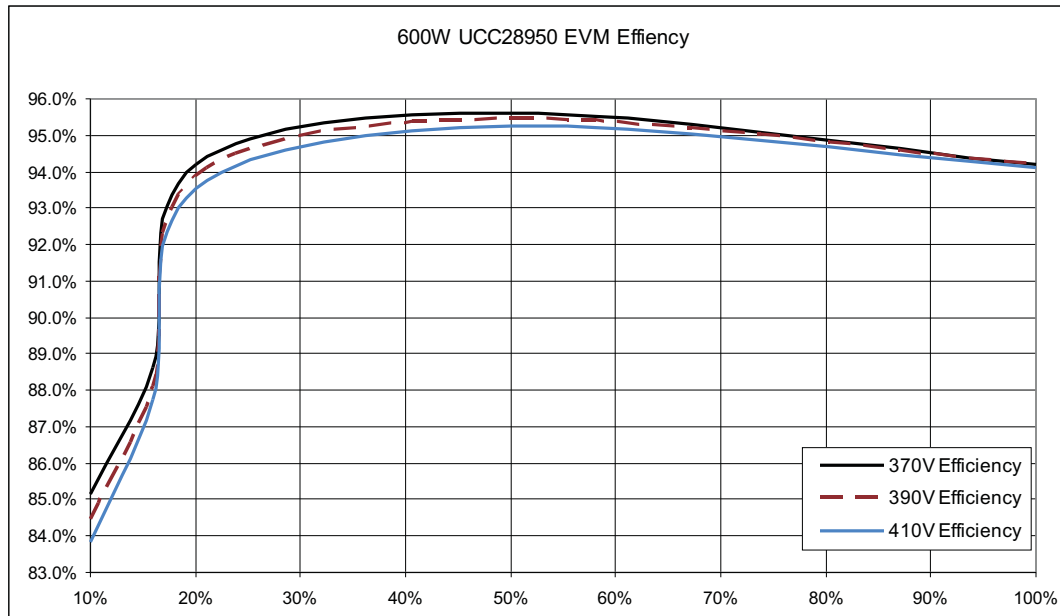
Figure 5. Efficiency 10% to 100% Load
