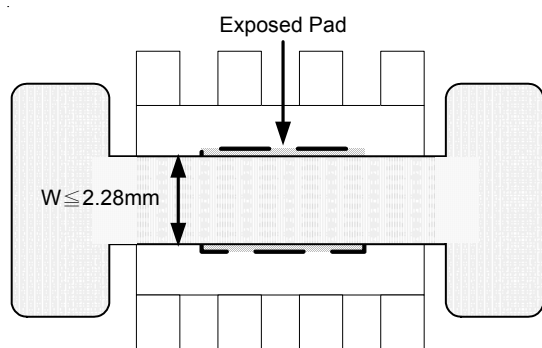
Figure 9. Dog-Bone layout
