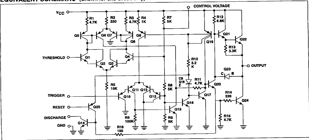
EQUIVALENT SCHEMATIC (Shown for one circuit only)
