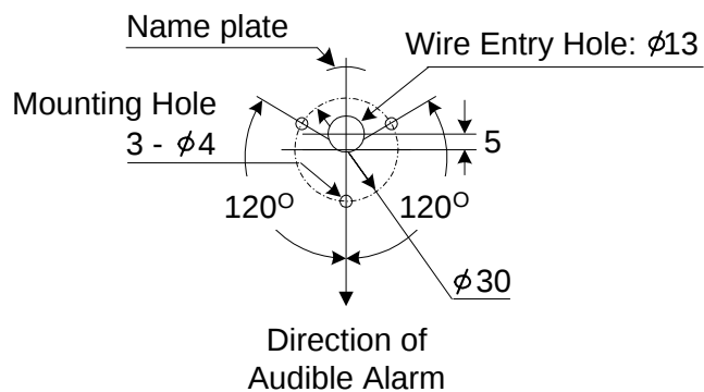
Mounting Dimensions
