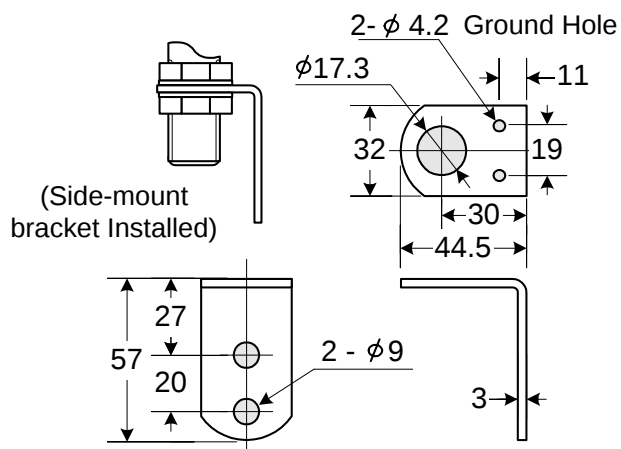
Side-mount Bracket (Supplied)
