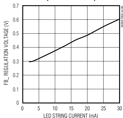
FB_ VOLTAGE vs. LED CURRENT (ANALOG DIMMING)
