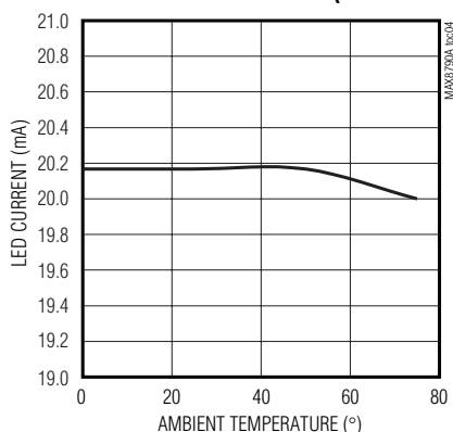
LED CURRENT vs. AMBIENT TEMPERATURE (BRT = 100%)
