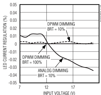
LED CURRENT REGULATION vs. INPUT VOLTAGE
