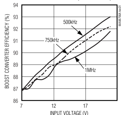
BOOST CONVERTER EFFICIENCY vs. INPUT VOLTAGE (BRT = 100%)
