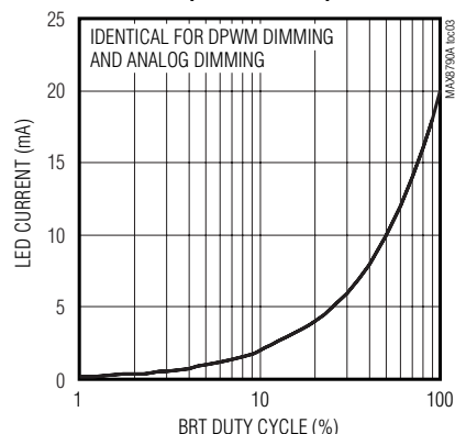
LED CURRENT vs. BRT DUTY CYCLE (BRT AT 200kHz)
