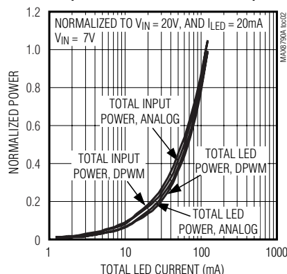
NORMALIZED POWER vs. TOTAL LED CURRENT (ANALOG AND DPWM DIMMING)
