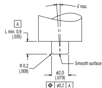
RECOMMENDED SHAPE OF ACTUATOR
