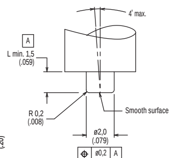
RECOMMENDED SHAPE OF ACTUATOR
