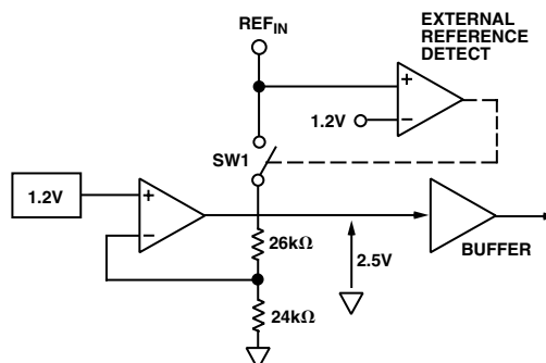
Figure 9. On-Chip Reference
