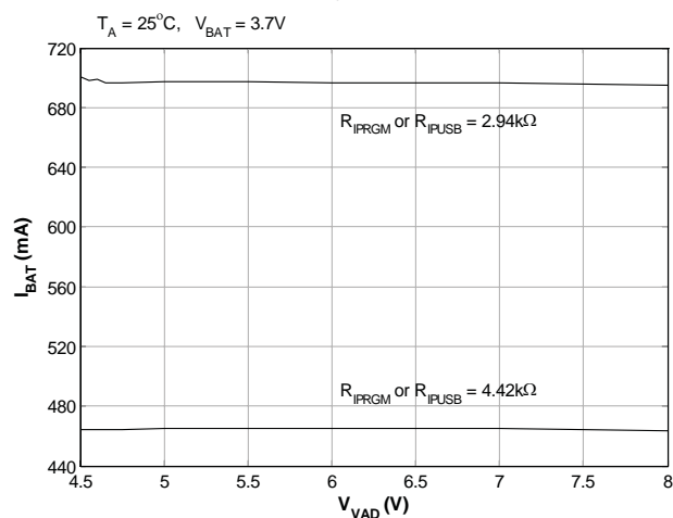
CC FQ Line Regulation (AD or USB)
