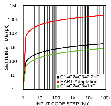
Figure 7. Settling Time vs Input Step Size
