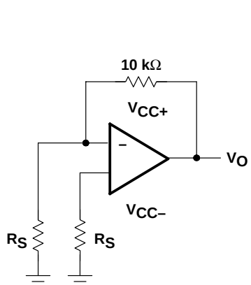
Figure 3. Noise-Voltage Test Circuit
