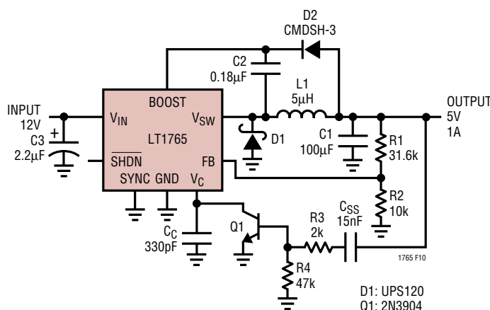
Figure 10. Buck Converter with Adjustable Soft Start
