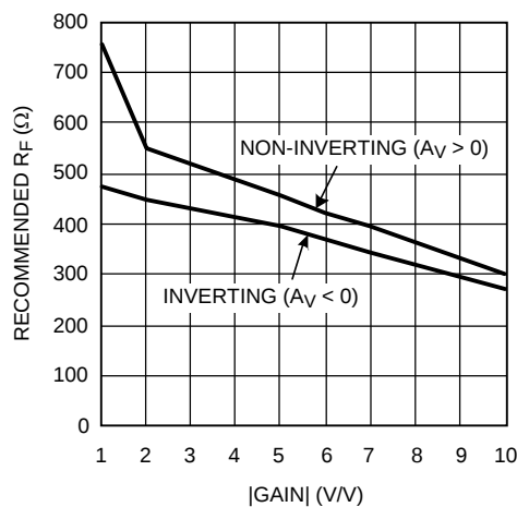
Figure 24. Recommended R_F vs. Gain
