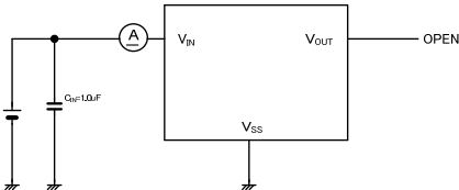
Circuit ③
