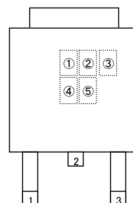
TO-252
