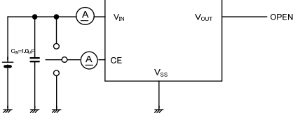
Circuit ②
