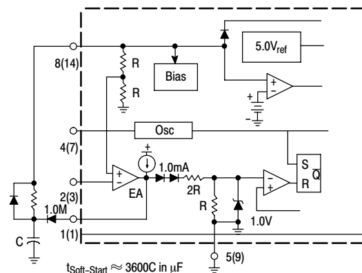
Figure 24. Soft-Start Circuit
