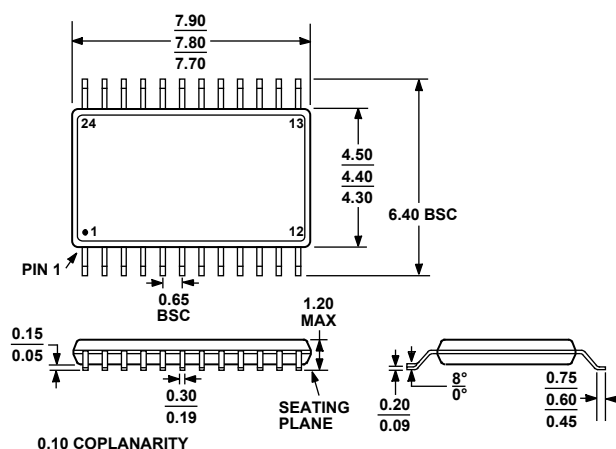
COMPLIANT TO JEDEC STANDARDS MO-153-AD Figure 45. 24-Lead Thin Shrink Small Outline Package [TSSOP] (RU-24) Dimensions shown in millimeters
