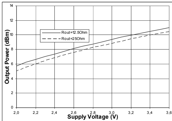
Figure 7. Output Power vs. Supply Voltage (PA=differential, R_{Ant+Matching}=422\Omega , cont. Tx)
