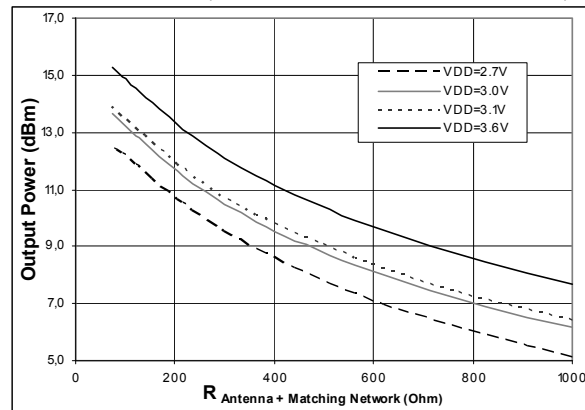
Figure 6. Output Power vs. Impedance of Antenna+Matching Network (PA=differential, R_{out}=12.5\Omega , cont. Tx)
