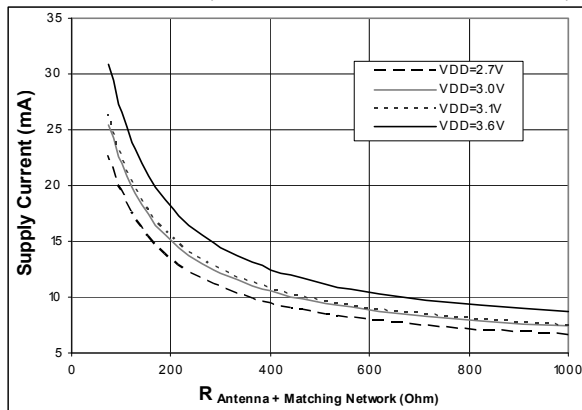
Figure 5. Supply Current vs. Impedance of Antenna+Matching Network (PA=differential, R_{out}=12.5\Omega , cont. Tx)
