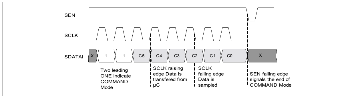
Figure 18. Single COMMAND byte
