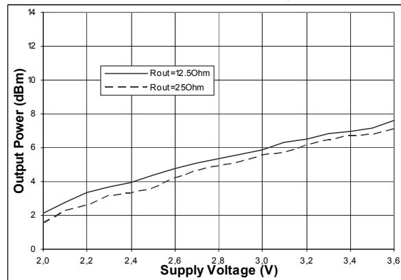
Figure 8. Output Power vs. Supply Voltage (PA=single ended, R_{Ant+Matching}=422\Omega , cont. Tx)
