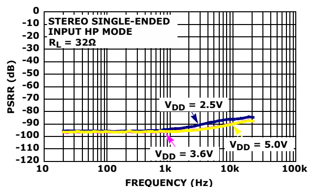
FIGURE 23. POWER SUPPLY REJECTION RATIO (HEADPHONES) vs FREQUENCY
