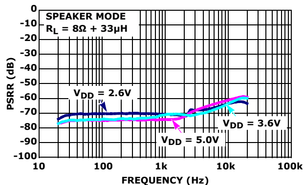
FIGURE 22. POWER SUPPLY REJECTION RATIO (SPEAKER) vs FREQUENCY
