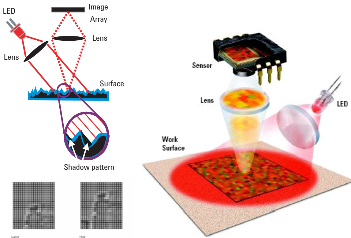
Figure 2. Illustration of Optical Navigation technology
