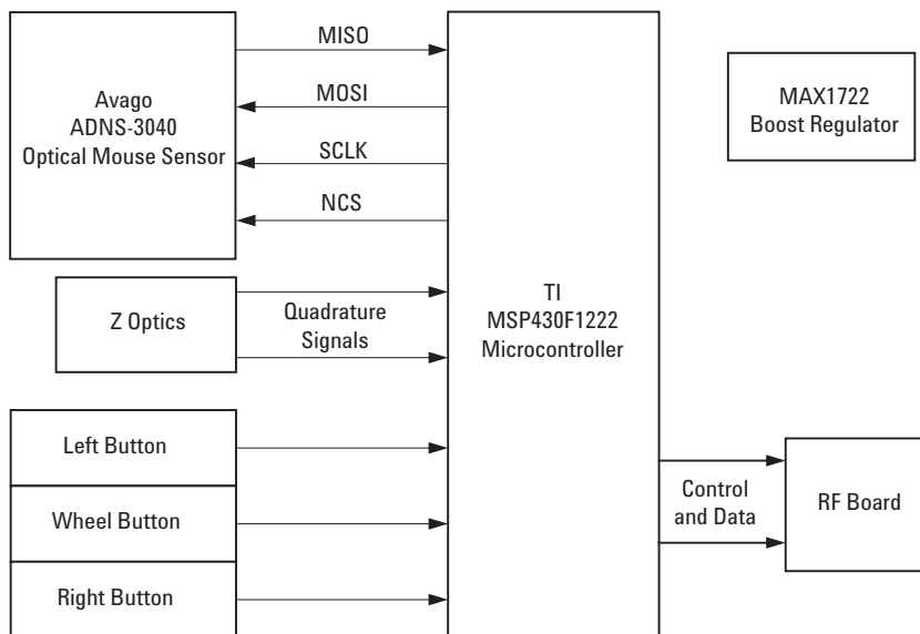
Figure 1. ADNK-3034-T127 Reference Design Mouse functional Block Diagram
