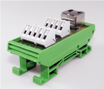
CIM/RJ45
